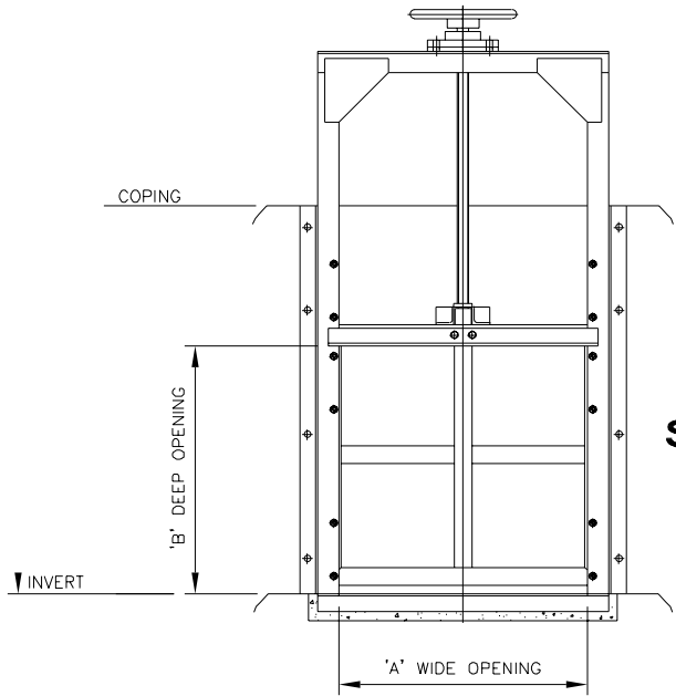
FRONT ELEVATION
